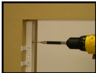
With hinge aligned, secure the top screw.
