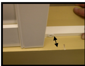
Adjust light block back or forward to bring panel flush with wall plain.
